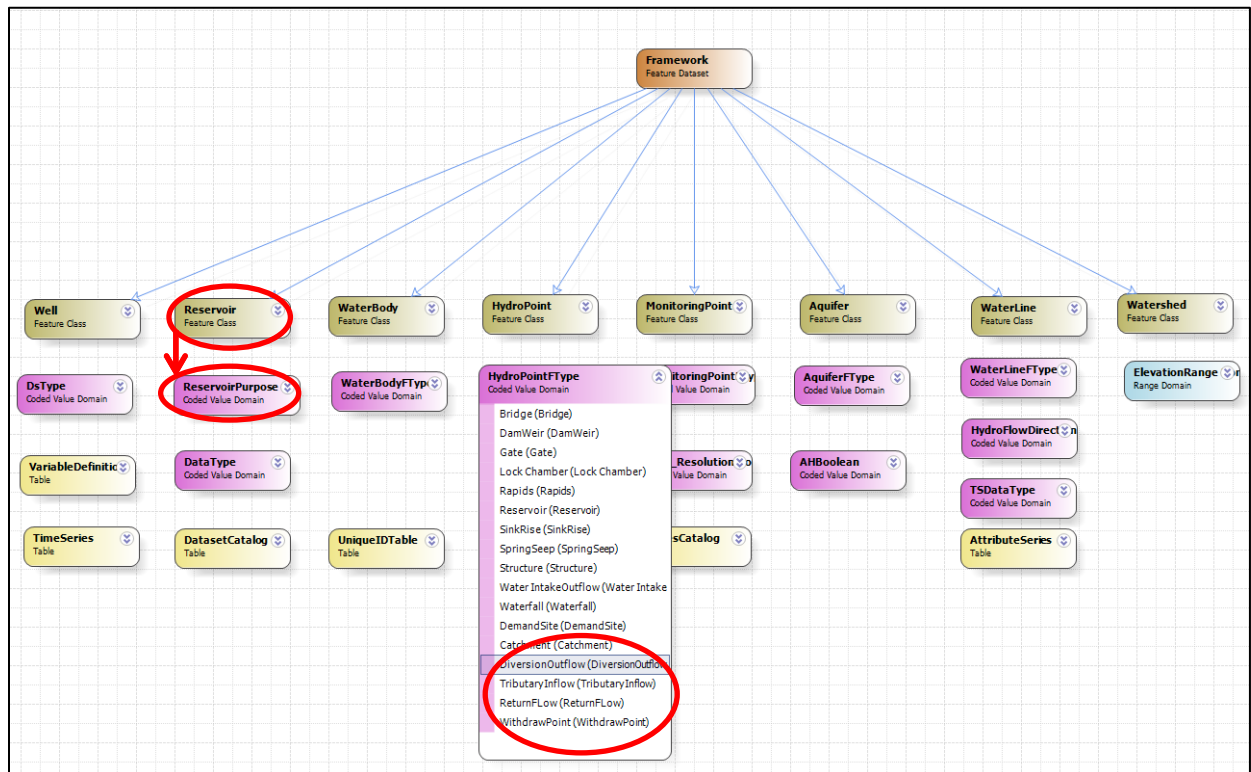
Figure 5: A snap shot of the modified geodatabase of Arc Hydro Framework using Arc Diagrammer software (ESRI, 2008)
