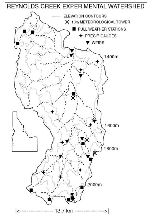
Figure 2: RCEW data acquisition and telemetry network.
